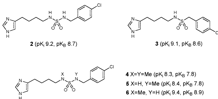
Figure 1. N -Methylation of JB96132 (pK i : g.p. cortex; pK B : g.p. ileum).
